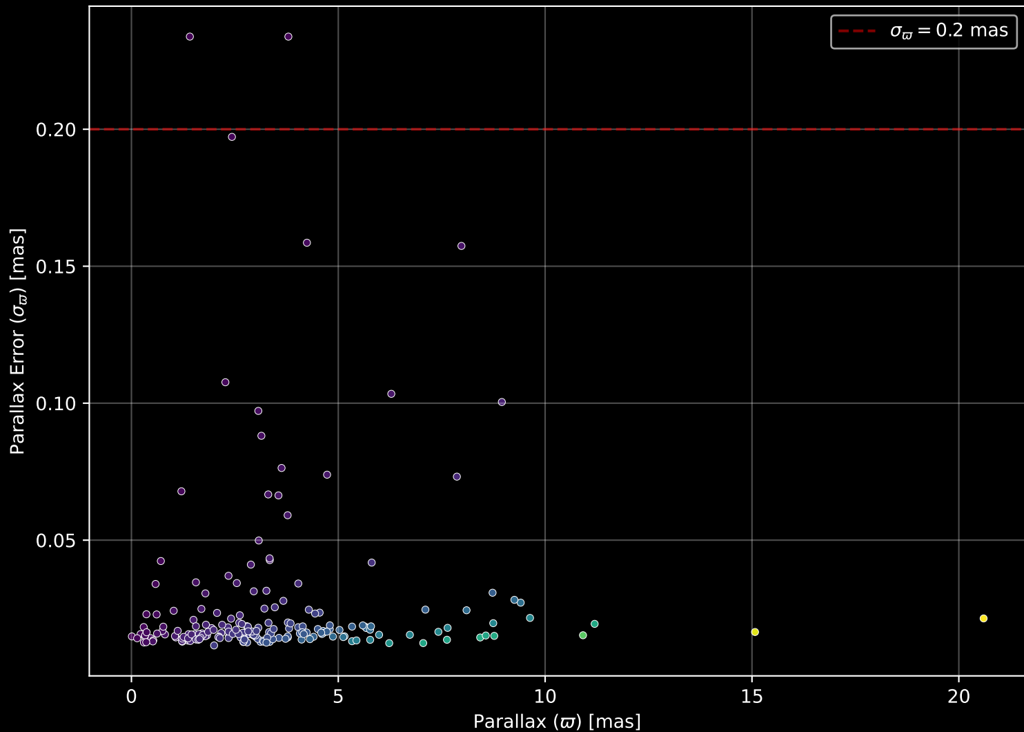
APOGEE DR17 Field: [139+74_MGA] Parallax Quality (n= 193)
