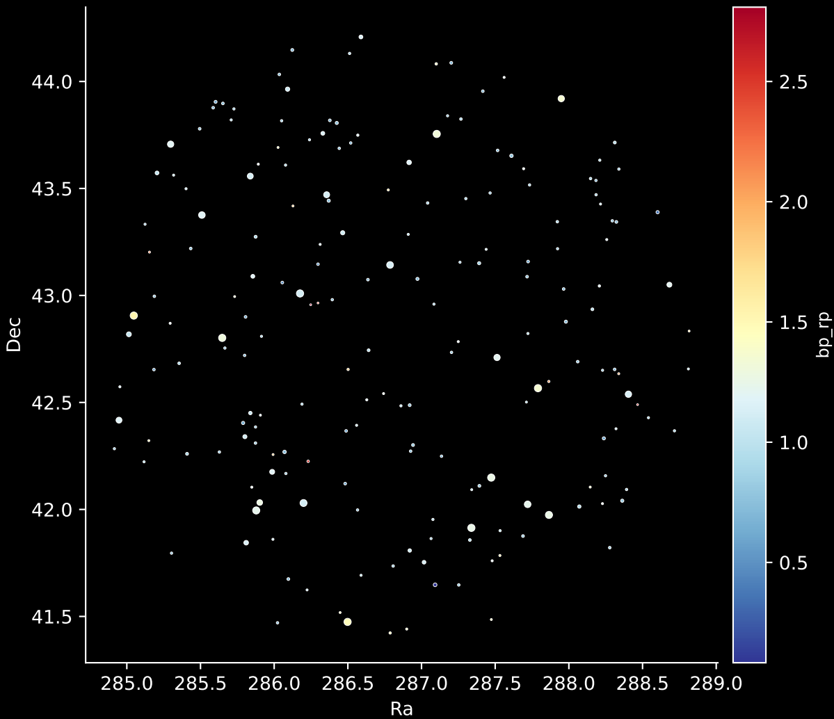
APOGEE DR17 Field: [139+74_MGA] Stars: 193
