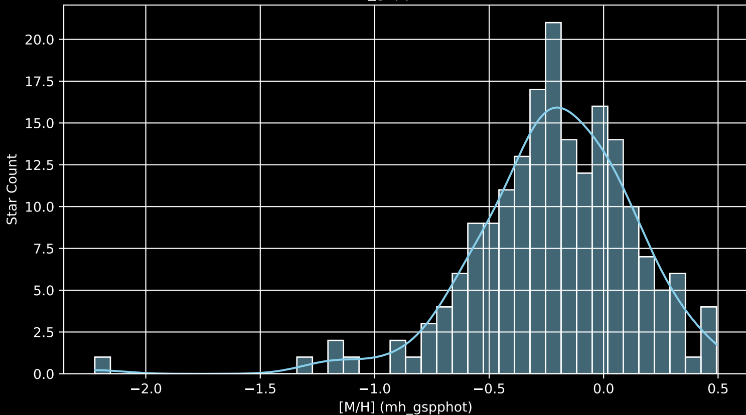
APOGEE DR17 Field: [139+74_MGA [M/H] (mh_gspphot) (n= 190)
