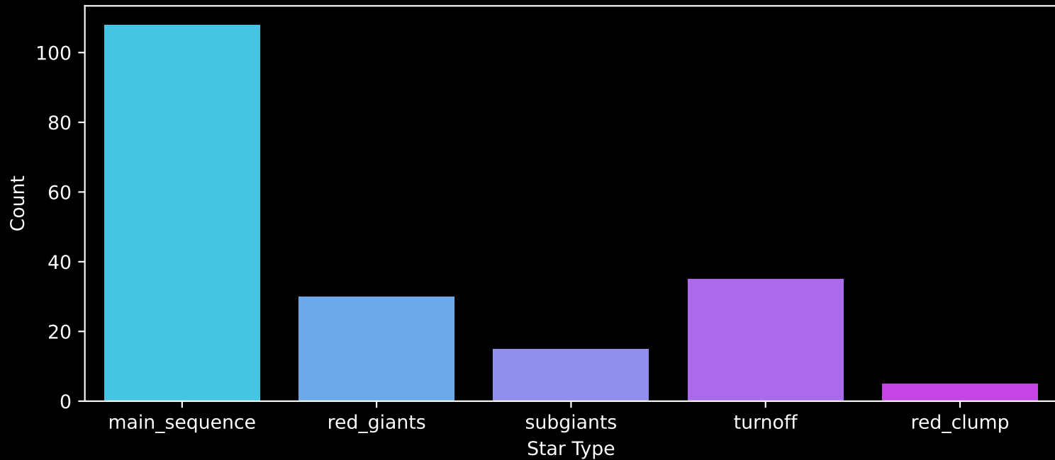
APOGEE DR17 Field: [139+74_MGA] Count plot of Star Type
