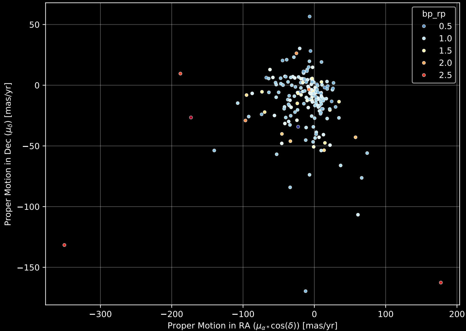
APOGEE DR17 Field: [139+74_MGA] Proper Motion Diagram (n= 193)
