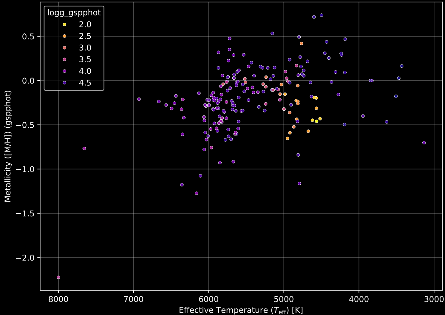
APOGEE DR17 Field: [139+74_MGA] Stellar Population Parameters (n= 193)
