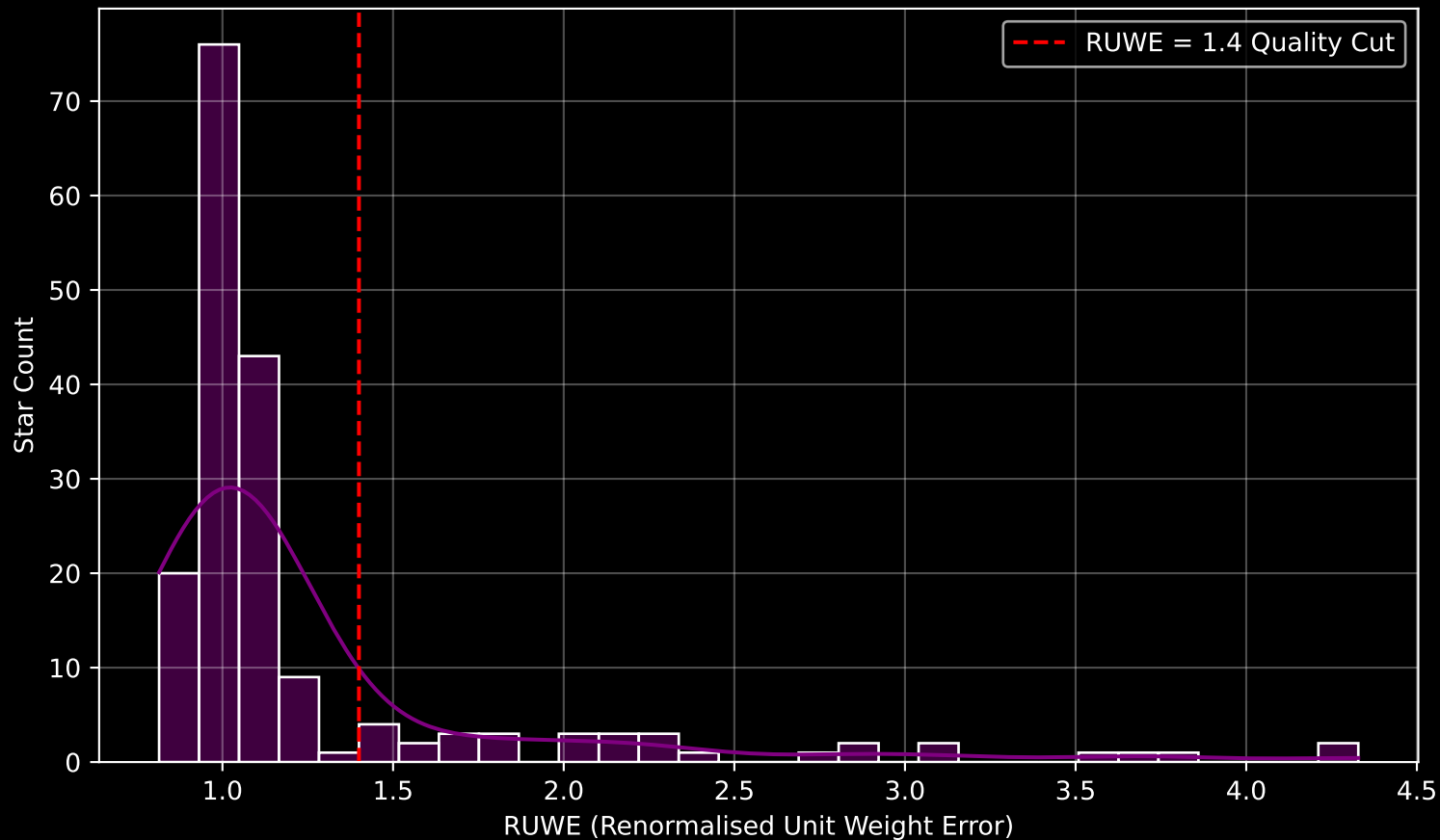
GAPOGEE DR17 Field [139+74_MGA] RUWE Distribution (n= 181)
